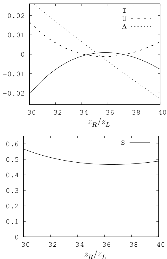
Figure 5: The numerical result of oblique correction parameters as the functions of z_R with z_L = z_i = 10^6 . The fine structure constant and the electroweak gauge boson mass are fitted to the experimental data.
